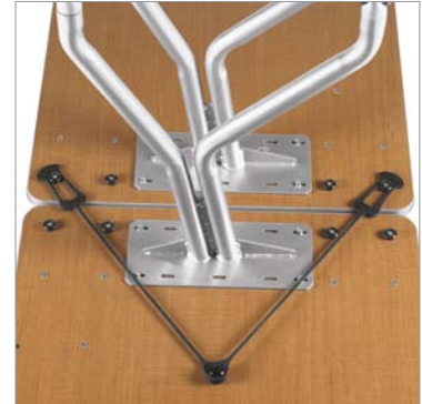
"Bungee Cords" connect tables securely and are included with all freestanding tables. The cords carry a lifetime warranty.
